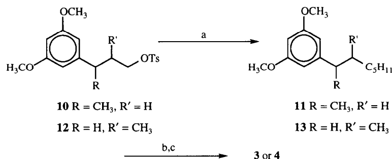
Scheme 1. (a) \text{Li}_2\text{CuCl}_4/\text{BuMgCl}/\text{THF} , -78^\circ to 25^\circ\text{C} ; (b) \text{BBr}_3/\text{CH}_2\text{Cl}_2 , 0^\circ to 25^\circ\text{C} ; (c) menthadienol/ \text{HOTs}/\text{C}_6\text{H}_6 , 80^\circ\text{C} .
