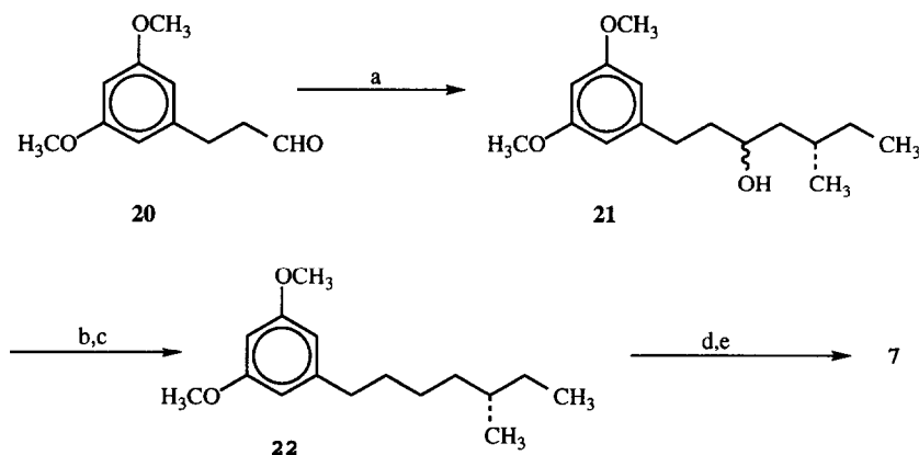
Scheme 4. (a) ( S )-CH 3 CH 2 CH(CH 3 )CH 2 MgBr, 25°C then 35°C; (b) TsCl/C 5 H 5 N/CHCl 3 , 0°C; (c) LiAlH 4 /ether, 35°C; (d) BBr 3 /CH 2 Cl 2 0° to 25°C; (e) p -menthadienol/HOTs/C 6 H 6 , 80°C.
