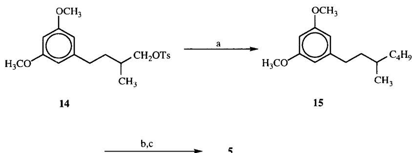
Scheme 2. (a) \text{Li}_2\text{CuCl}_4/\text{PrMgBr}/\text{THF} , -78^\circ to 25^\circ\text{C} ; (b) \text{BBr}_3/\text{CH}_2\text{Cl}_2 , 0^\circ to 25^\circ\text{C} ; (c) menthadienol/ \text{HOTs}/\text{C}_6\text{H}_6 , 80^\circ\text{C} .
