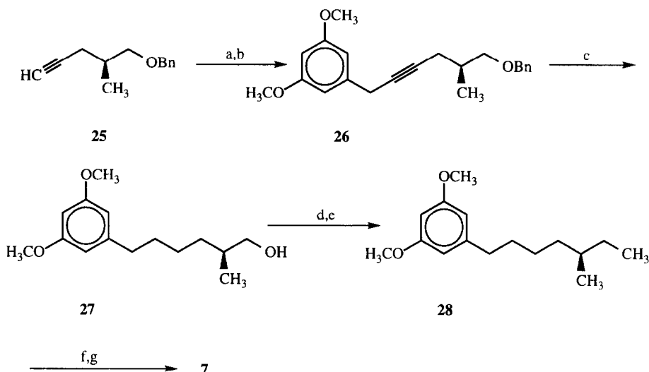
Scheme 5. (a) BuLi/THF, 0 to 25 °C; (b) 3,5-dimethoxybenzyl bromide/THF, then LiI, reflux; (c) H 2 (g) 10% Pd(C)/EtOH/45 psi; (d) TsCl/C 5 H 5 N/CHCl 3 , 0 °C; (e) Li 2 CuCl 4 /MeMgBr/THF, -78° to 25 °C; (f) BBr 3 /CH 2 Cl 2 , 25 °C; (g) p -menthadienol/HOTs/C 6 H 6 , 80 °C.
