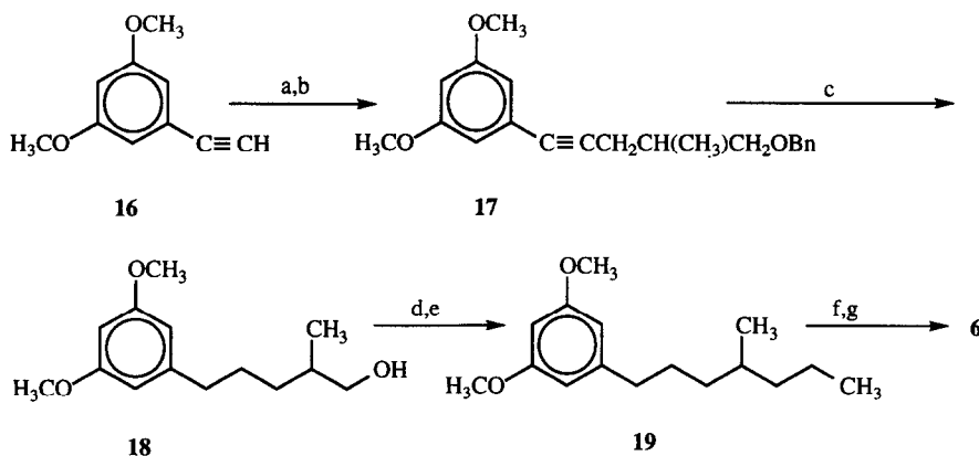
Scheme 3. (a) BuLi/THF, 0°C; (b) 3-benzyloxy-1-bromo-2-methylpropane/THF/DMSO, 0°C then 25°C; (c) H 2 (g)/10% Pd(C)/EtOH/45 psi; (d) TsCl/C 5 H 5 N/CHCl 3 , 0°C; (e) Li 2 CuCl 4 /EtMgBr/THF, -78° to 20°C; (f) BBr 3 /CH 2 Cl 2 , 0° to 25°C; (g) p -methadienol/HOTs/C 6 H 6 , 80°C.
